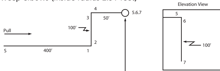
Figure 7-17 Conduit Layout
