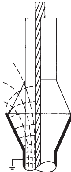
Fig. 8-2 Dielectric Field - Receding Ground Plane - Stress Relief Cone
