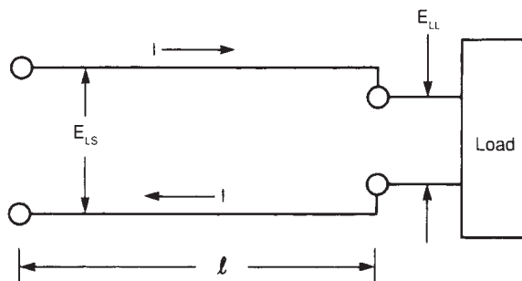
Figure 6-3 AC Single-Phase, Two-Wire Circuit
