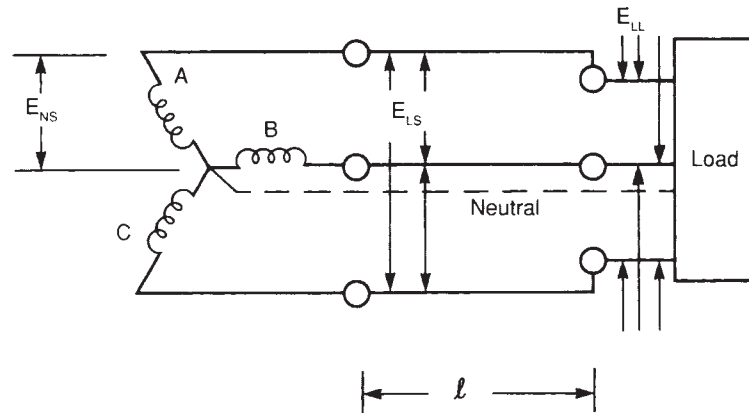
Figure 6-4 AC Three-Phase, Y (Wye) Circuit
