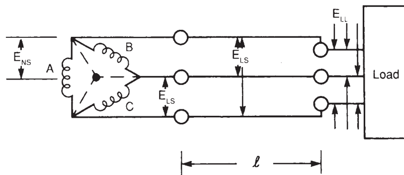
Figure 6-4 AC Three-Phase, Y (Wye) Circuit
