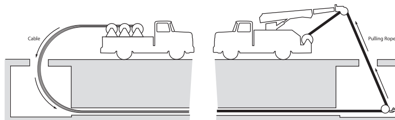
Figure 7-1 Pulling Cable in Duct
