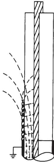
Fig. 8-3 Dielectric Field-Voltage Gradient (Material)-Stress Relief
