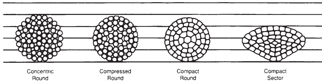
Figure 2-1 Comparative Sizes and Shapes of 61 Strand Conductors
