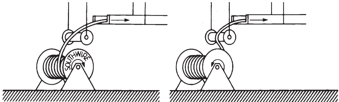
Figure 7-6 Sheave Arrangements for Feeding into Cable Tray
