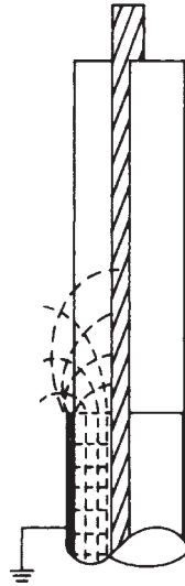
Fig. 8-1 Dielectric Field - No Stress Relief
