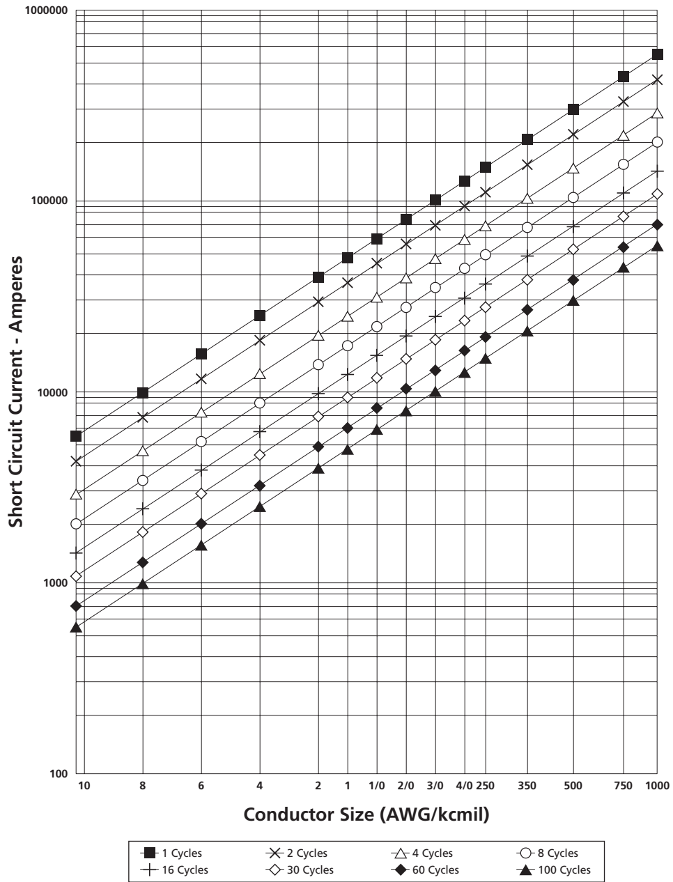
Figure 6-16 Allowable Short Circuit Currents for Thermoplastic Insulated Copper Conductors Rated 90°C Maximum Continuous Operation
