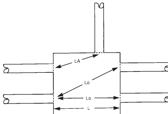
Figure 7-12 Pull Box Dimensions
