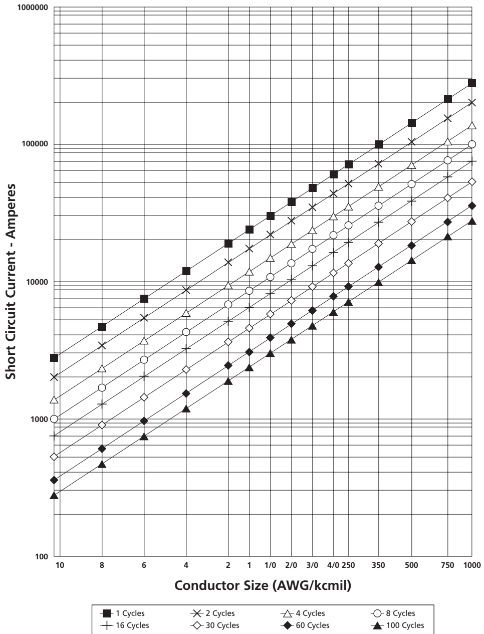
Figure 6-18 Allowable Short Circuit Currents for Thermoplastic Insulated Copper Conductors Rated 75°C Maximum Continuous Operation
