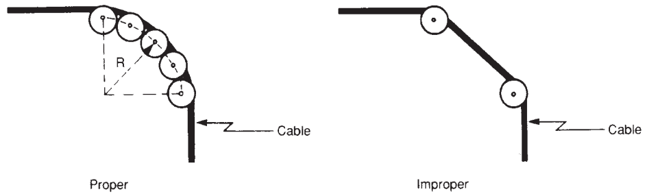
Figure 7-5 Multiple Sheaves
