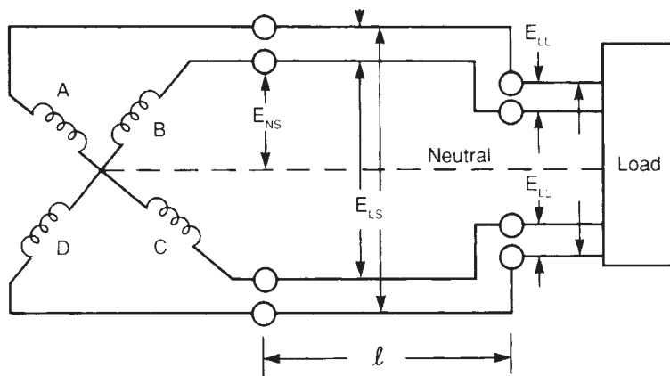
Figure 6-6 AC Two-Phase, Four- or Five-Wire Circuit
