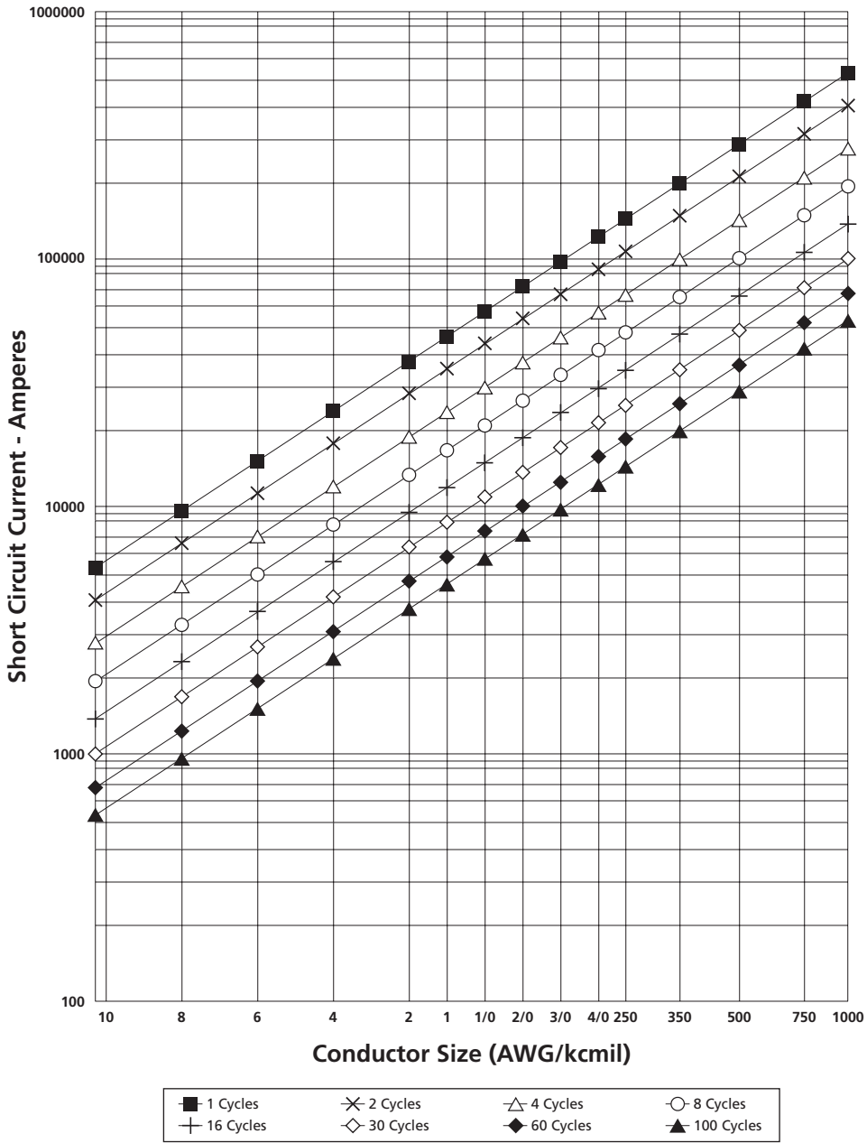
Figure 6-17 Allowable Short Circuit Currents for Thermoplastic Insulated Copper Conductors Rated 105°C Maximum Continuous Operation
