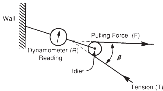
Figure 7-11 Variables for Dynamometer Correction Equation
