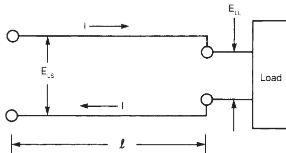
Figure 6-1 DC Two-Wire Circuit
