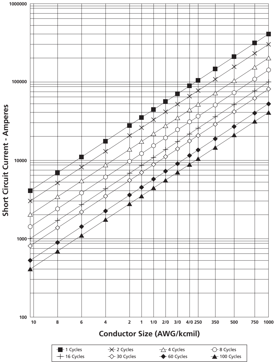
Figure 6-15 Allowable Short Circuit Currents for Thermoplastic Insulated Copper Conductors Rated 75°C Maximum Continuous Operation
