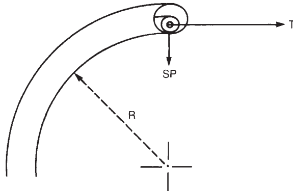
Figure 7-15 Sidewall Pressure Factors
