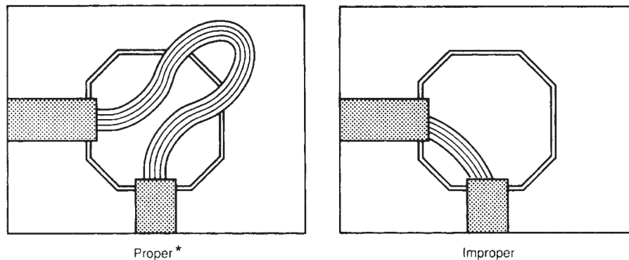
Figure 7-10 Pull-Through Enclosure
