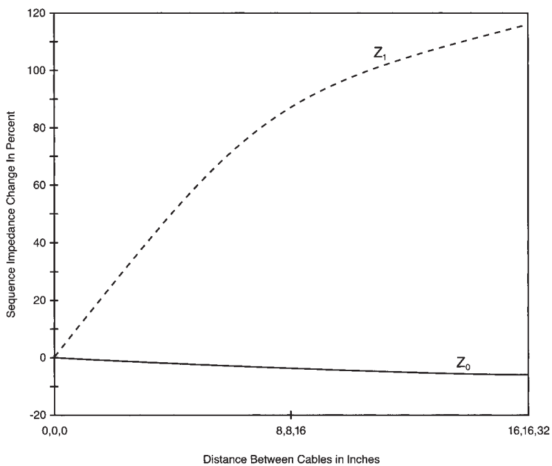
Figure 6-24 Effect of Cable Spacing on Sequence Impedance
