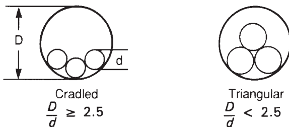
Figure 7-13 Configuration of Three Single Conductors
