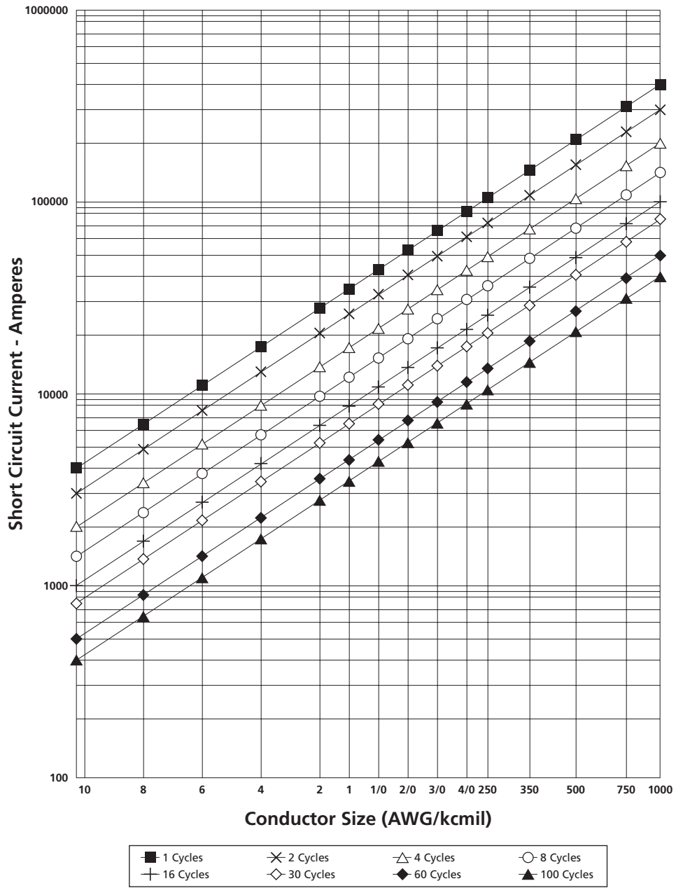
Figure 6-15 Allowable Short Circuit Currents for Thermoplastic Insulated Copper Conductors Rated 75°C Maximum Continuous Operation
