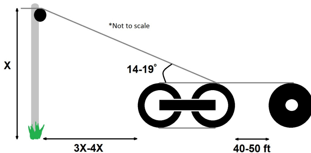
Figure 11. Orientation for bullwheel/payoff setup.
