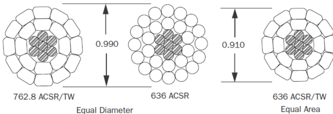
Figure 1. Comparison of ACSR and ACSR/TW conductors.
